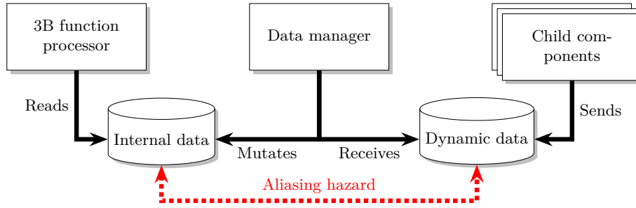
Fig. 4. Shared data snapshots.
