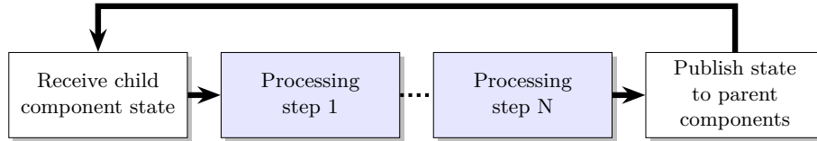
Fig. 3. The 3B function processing event loop.
